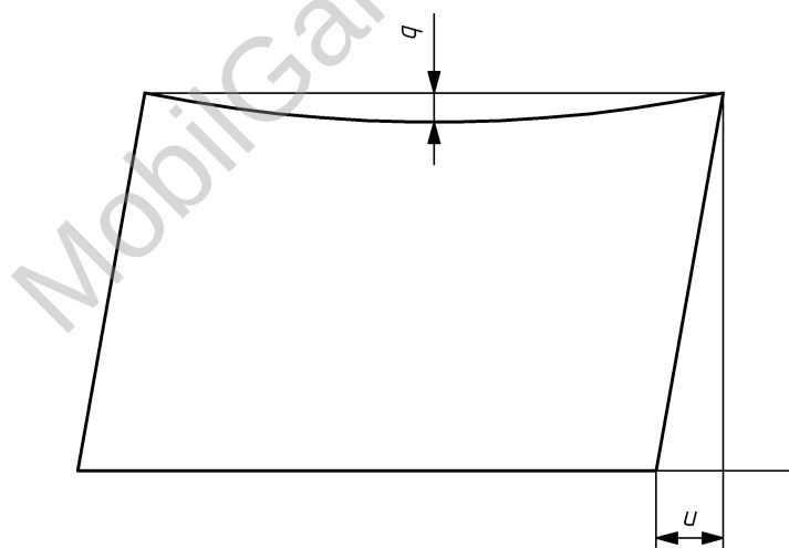
Figure 1 — Out-of-squareness u and edge camber q
